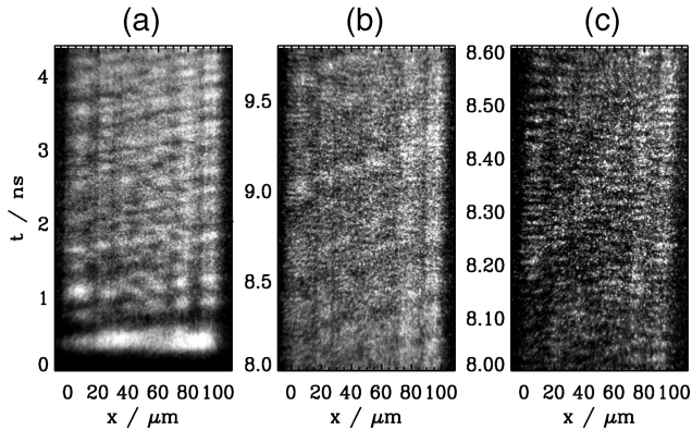
Fig. 1. Spatiotemporal emission dynamics of the near field of the solitary laser at I_{\text{pump}} = 1.75I_{\text{thr}} : (a) Turn-on behavior in a 4.4-ns-long time window, (b) behavior 8 ns after turn-on in a 1.8-ns-long time window, and (c) behavior in a 600-ps-long time window.
