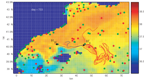
(a) Day 733. The unstable manifold of H_W does not appear to intersect the stable manifold of H'_E . The unstable manifold is strongly influenced by the circulation associated with the elliptic ISP immediately to the lower right of H'_E .
