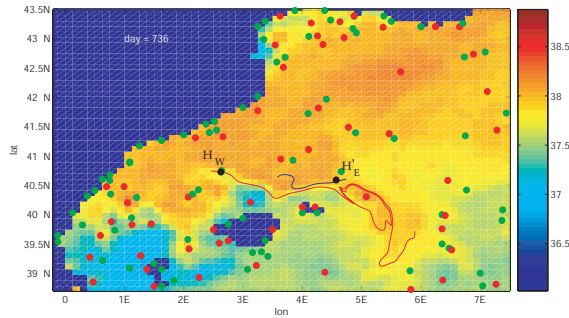
(b) Day 736. As the elliptic ISP moves further away from H'_E its influence carries the unstable manifold with it.
