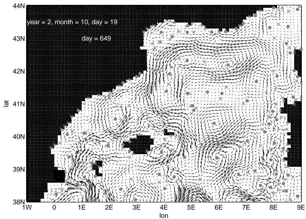
Figure 1: Velocity field at 16 m depth in the Northwestern Mediterranean at simulation day 649 (October). The Westernmost coast is the Spanish one, the islands are the Balearics, and the Easternmost coasts are portions of Corsica and Sardinia. Circles indicate elliptic ISPs and crosses indicate saddle-type ISPs.
