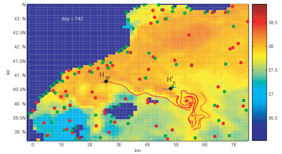
(c) Day 742. The earlier Lagrangian barrier now appears completely destroyed as a result of the influence of the eddy.
