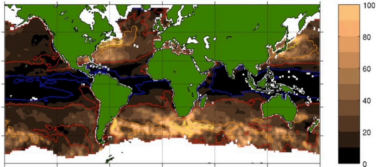
Figure 1: Contribution (in %) of intrinsic/chaotic ocean processes in the interannual variance of Sea Level Anomaly (a) and SST (b), as estimated from global eddying ocean simulations (Penduff et al, 2011).
