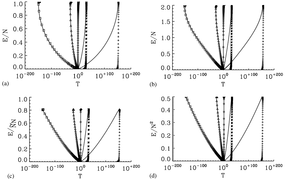
Fig. 1. Internal energy E as a function of the temperature T for the Ising model defined by (2) in the cases: (a) \alpha = \infty , d = 1 , (b) \alpha = \infty , d = 2 , (c) \alpha = 0.8 , d = 1 and (d) \alpha = 0 . The number of spins is N = 1000 . Solid lines are the results obtained in the microcanonical ensemble, while symbols correspond to the canonical ensemble. For the curves, from left to right, the values of q are q = 0.5, 0.9, 1, 1.1 , and 1.5 .
