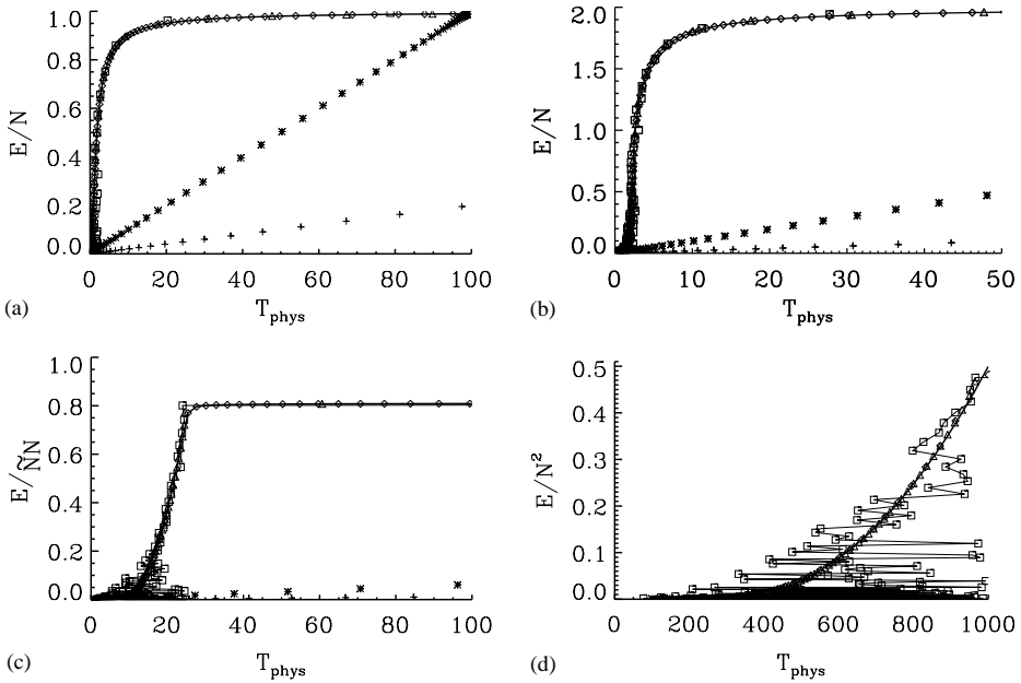
Fig. 2. Internal energy E as a function of the physical temperature T_{phys} . Same cases and symbol meanings as in Fig. 1.
