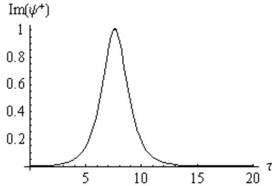
FIGURE 2. Numerical solution \text{Im}(\psi^+) versus \tau of system Eqs. (47a, 47b, 47c, 47d) integrated in the complex plane. The initial conditions are H^+(0) = 10^{-3}i , H^-(0) = 10^{-3}i , \psi^+(0) = 1 , \psi^-(0) = 1 .
