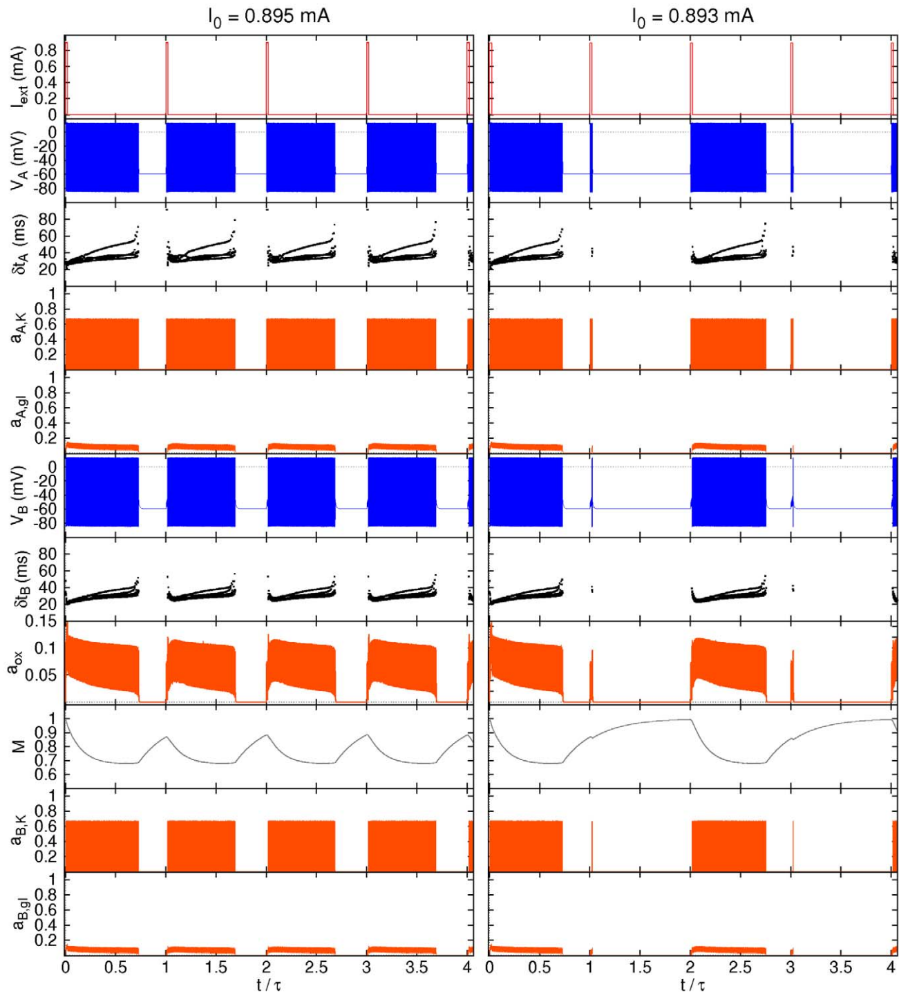
Figure 2. Response of the two-neuron model. Main variables and inter-spike times \delta t_p ( p = A, B ) versus time for a pulse height I_0 = 0.895 mA (left) and I_0 = 0.893 mA (right), see text for details. doi:10.1371/journal.pcbi.1002650.g002
