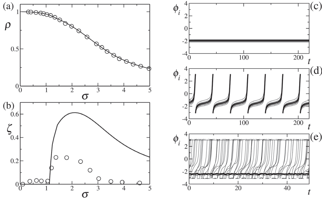
Fig. 2. Common firing in the active-rotator model. In panel (a) we show the Kuramoto order parameter \rho as a function of the diversity \sigma for the active-rotator model with quenched disorder defined in Eqs. 3.1. The parameters are \omega = 0.95 , C = 4 , N = 400 and the values of \eta_i are taken from a Gaussian distribution of zero mean and variance \sigma^2 . The line is the mean-field prediction obtained by solving the self-consistent equation (3.7) and the dots are the results of numerical simulations of the dynamical equations (3.1). Panel (b) plots the Shinomoto-Kuramoto order parameter \zeta as a function of diversity. A transition to a state in which the units pulse synchronously can be observed by the non-zero value of \zeta starting around \sigma = 1.164 . The line is the theoretical prediction Eq. (3.10) and the dots come from the numerical simulations. In the right panels, we show some representative trajectories \phi_i(t) (thin lines) and the average phase \Psi(t) (thick line) in the case of \sigma = 0.63 (panel c), \sigma = 1.73 (panel d) and \sigma = 3 (panel e). Note the transition from the quiescent state (c) to a situation of common pulsing (d) and then to incoherent pulsing (e).
